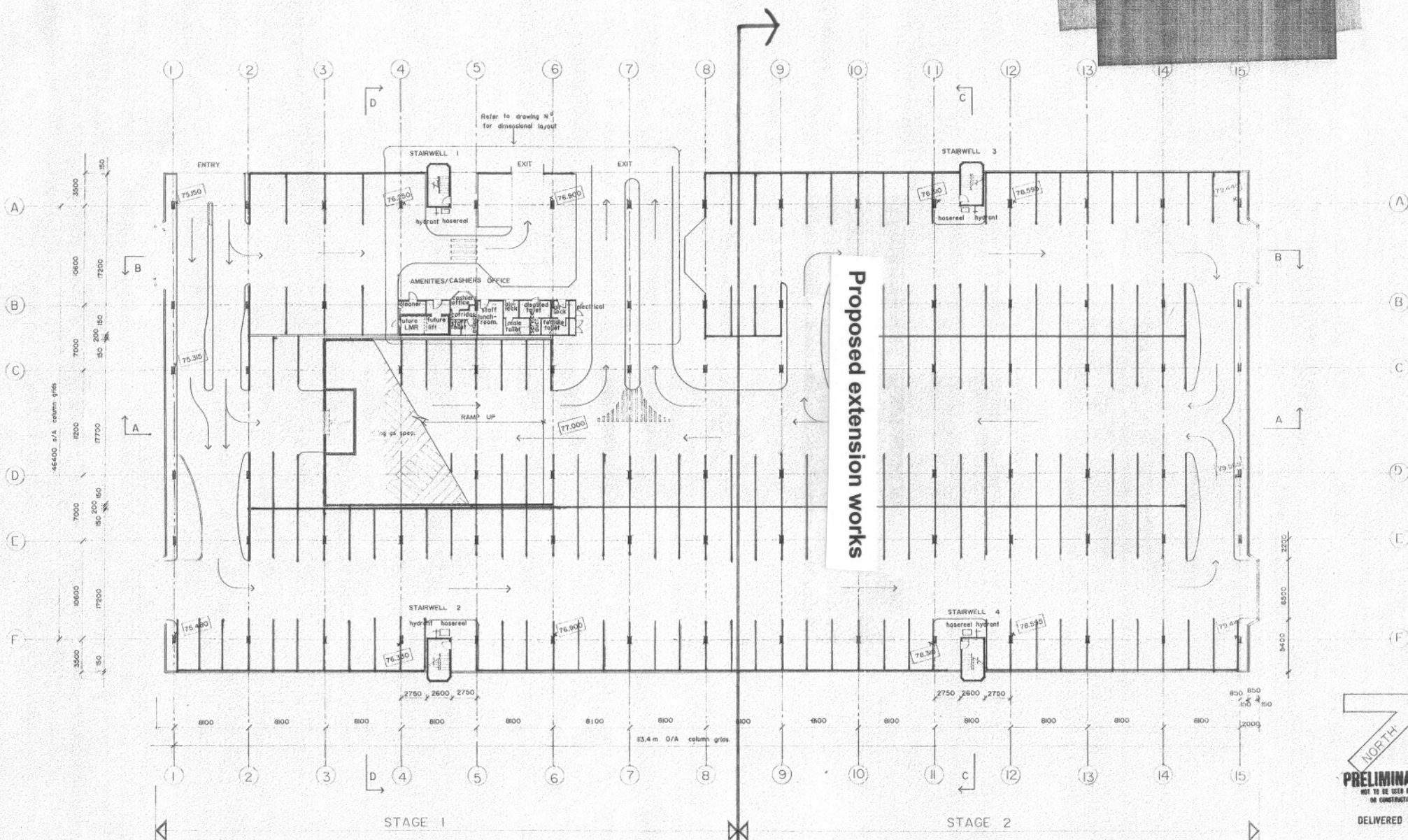
GROUND LEVEL FLOOR PLAN
