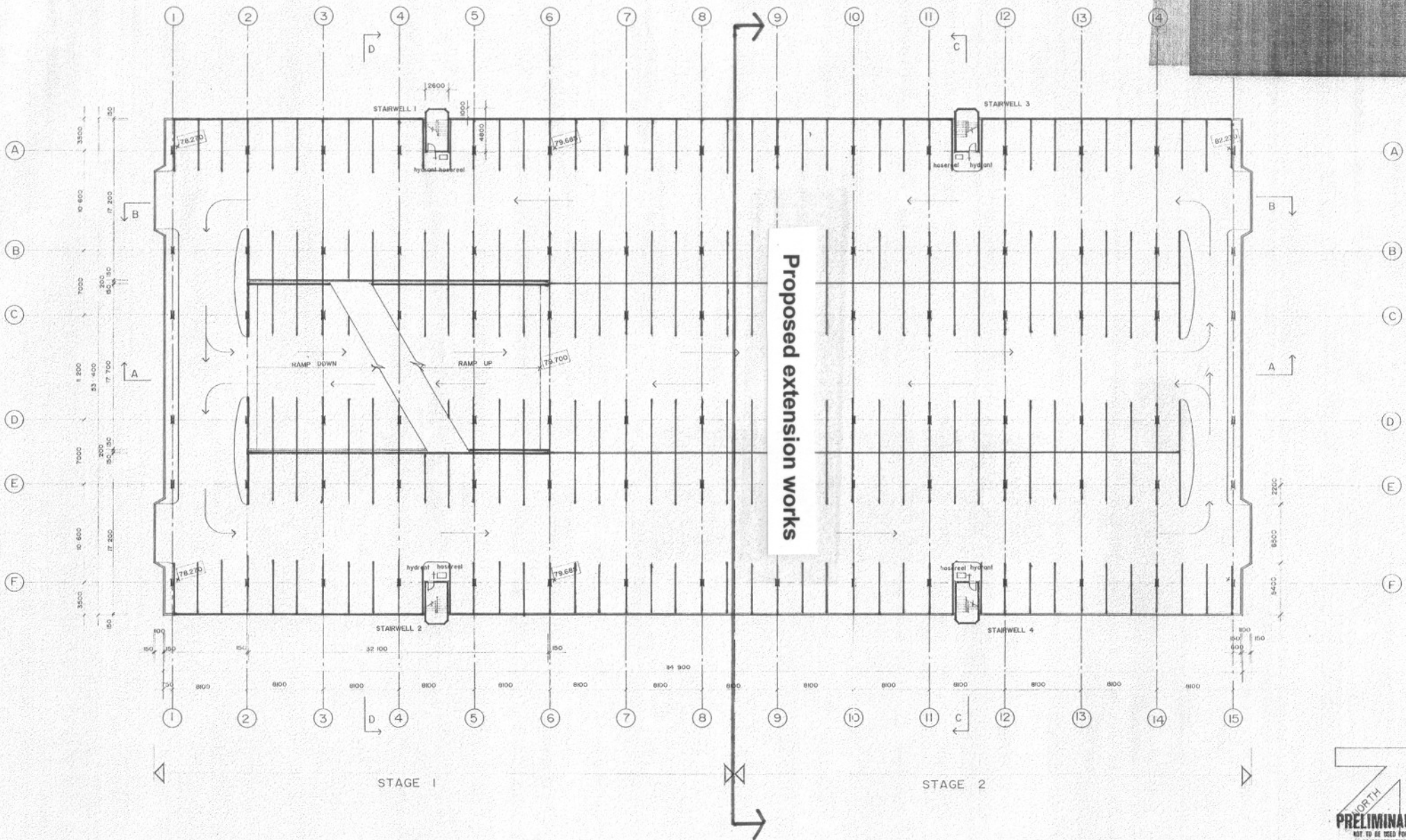
LEVEL I FLOOR PLAN
