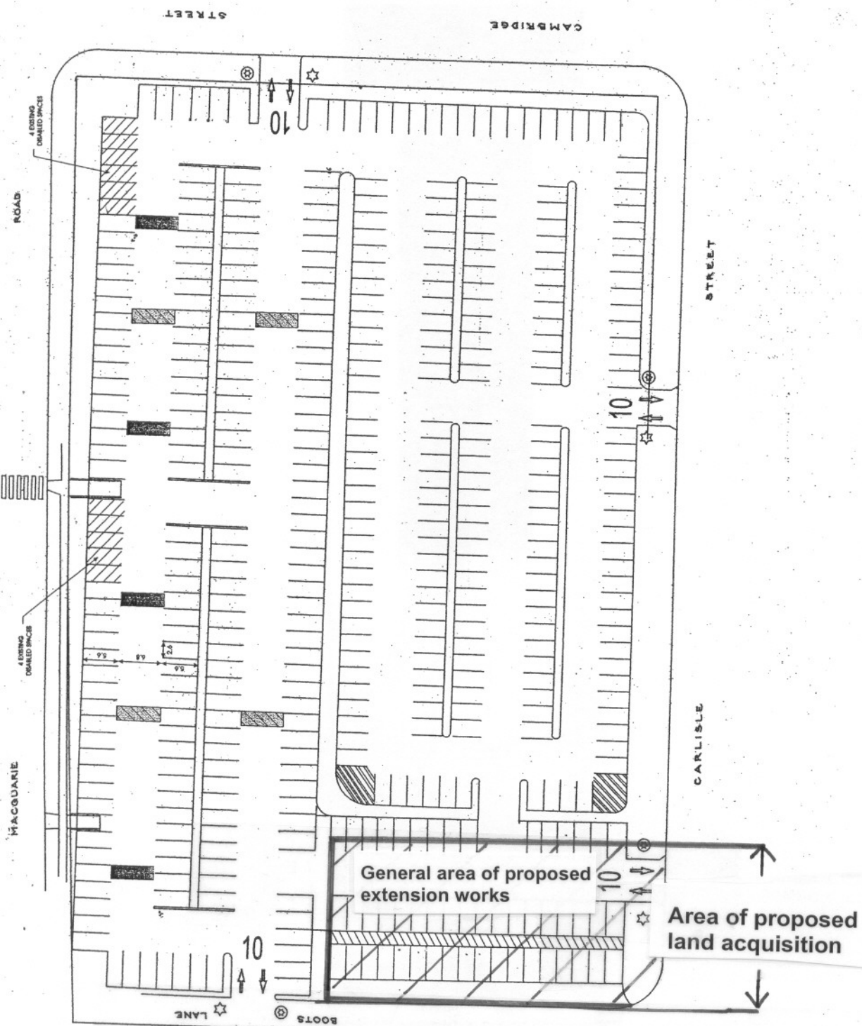
Appendix 7 Preliminary design of proposed extension to existing ground level public car parking facility at Boots Lane Ingleburn
