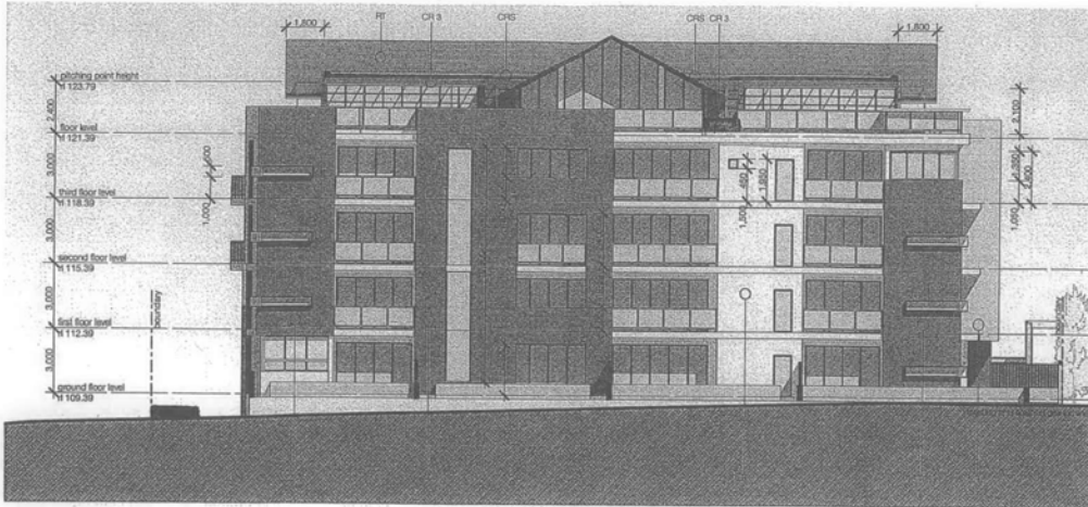
01 | north-west elevation
