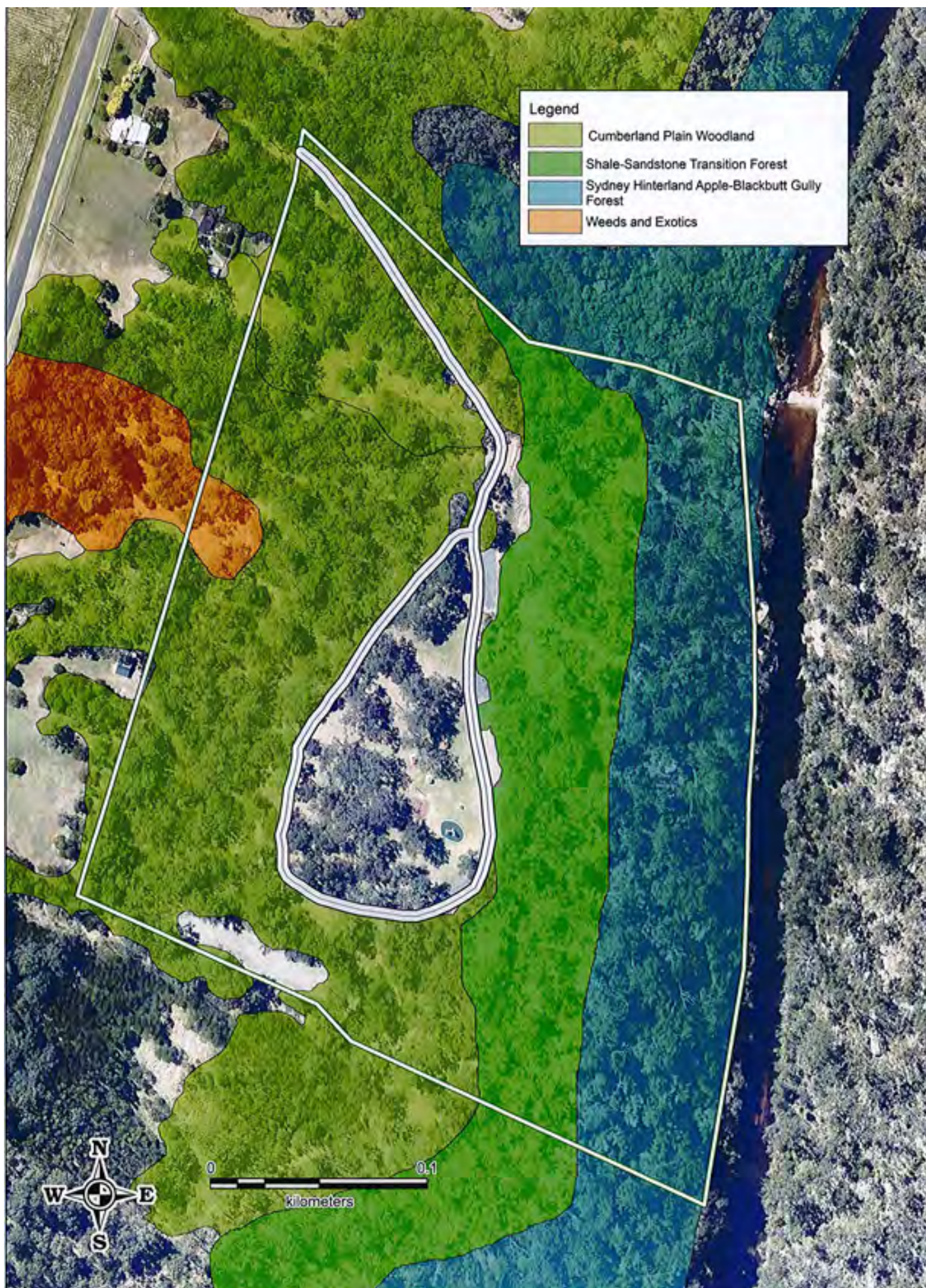
Figure 3: Vegetation Communities (SMA, Vegetation Mapping, OEH 2013)
